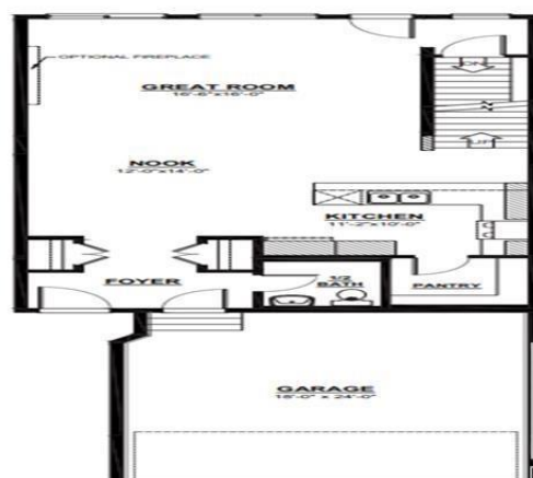
MAIN FLOOR 902 Sq. Ft. | 9 Ft. ceiling
